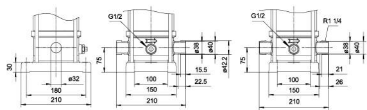
THREADED CONNECTOR(SMVS)/G CLAMP CONNECTOR(SMVS)/K
