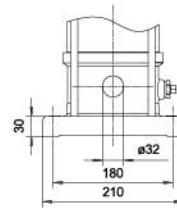
THREADED CONNECTOR(SMVS)/G
