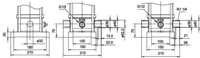
THREADED CONNECTOR(SMVS)/G CLAMP CONNECTOR(SMVS)/K
