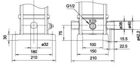
THREADED CONNECTOR(SMVS)/G
