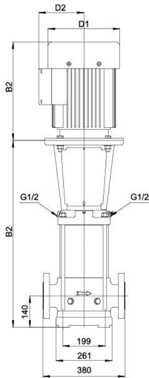
SMVS90/F
